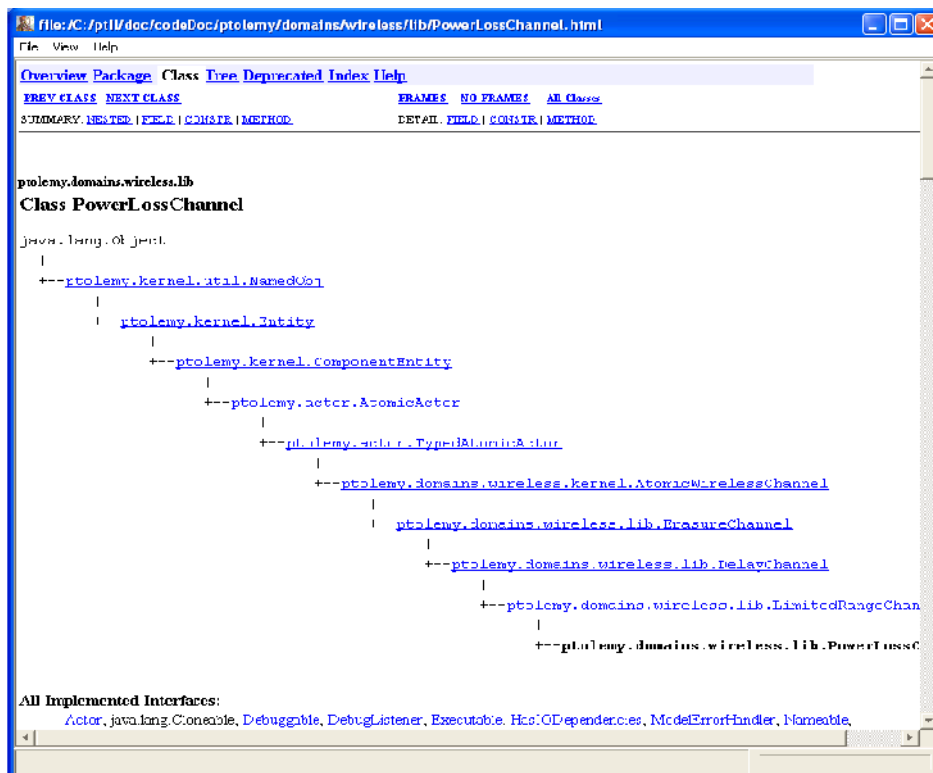
شکل (26) PowerLossChannel documentation
